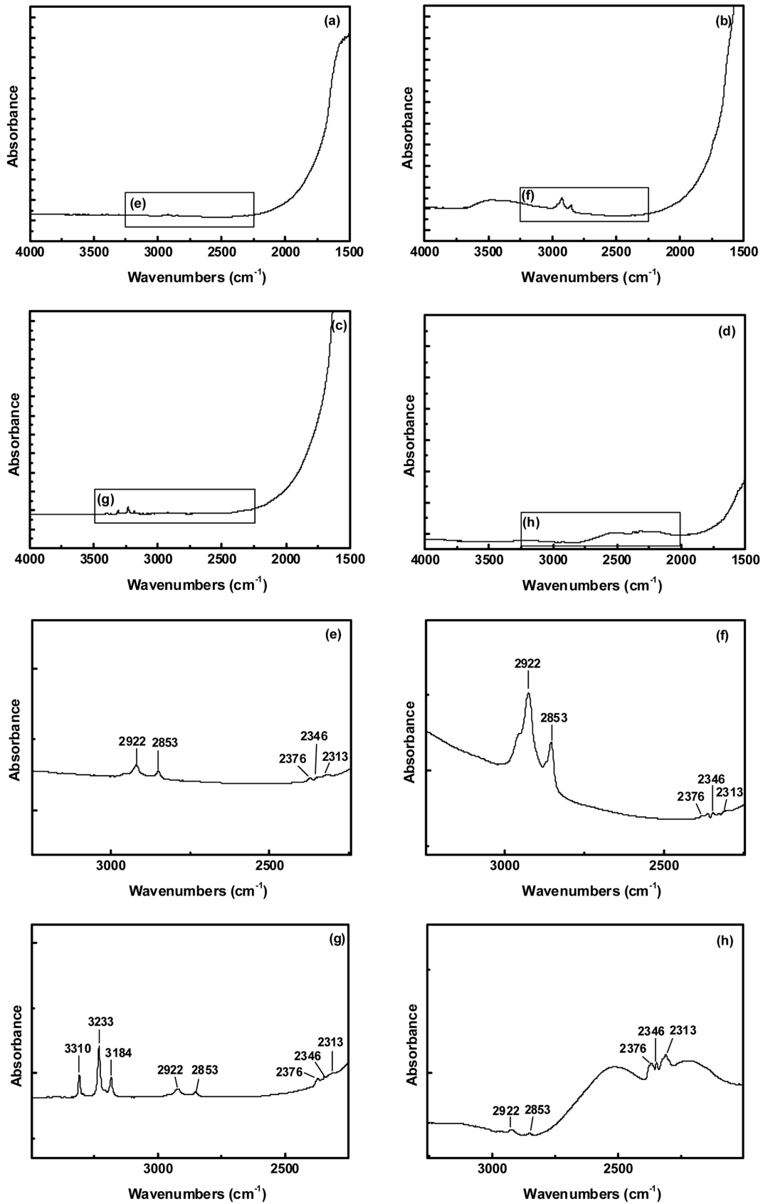
Fig. 6. FT-IR absorption spectra of 1500–4000 \text{cm}^{-1} in the region (a–d), enlarged spectra of 2250–3250 \text{cm}^{-1} in the region (e–g); (a) natural ruby, (b) flux synthetic ruby (platinum crucible), (c) verneuil synthetic ruby, (d) synthetic ruby in this study (alumina crucible), (e) enlarged spectra of (a), (f) enlarged spectra of (b), (g) enlarged spectra of (c), (h) enlarged spectra of (d).
