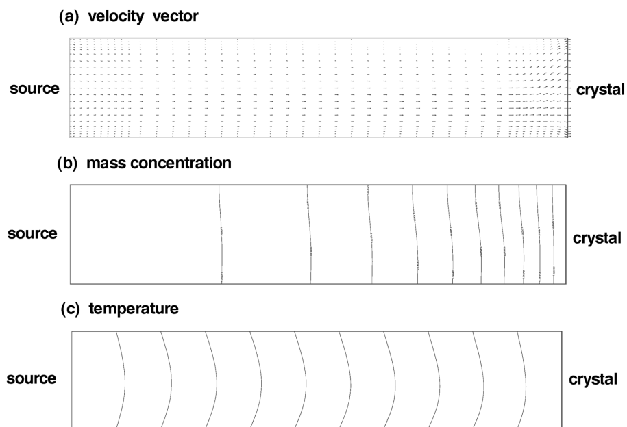
Fig. 4. Dimensionless velocity vector fields, temperature and mass concentration contours corresponding to the case of g_y = 0.1g_0 in Fig. 2. The maximum magnitude of the velocity vector is 0.12 \text{ cm s}^{-1} .
