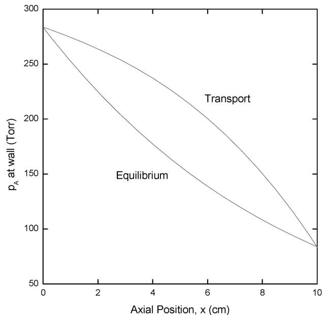
Fig. 7. Axial distribution of partial pressure of component A at the walls resulting from purely diffusive transport for Ar= 5 and the linear wall temperature profile between T_s = 612.5 K and T_c = 576.0 K. The equilibrium vapor pressure profile corresponding to the wall temperature distribution is shown for the purpose of comparison. Based on Ar = 5.0, Pr = 0.8, Le = 0.37, Gr_i = 0 , Gr_s = 0 , Pe = 2.27, Cv = 1.1, g_y = 0 .
