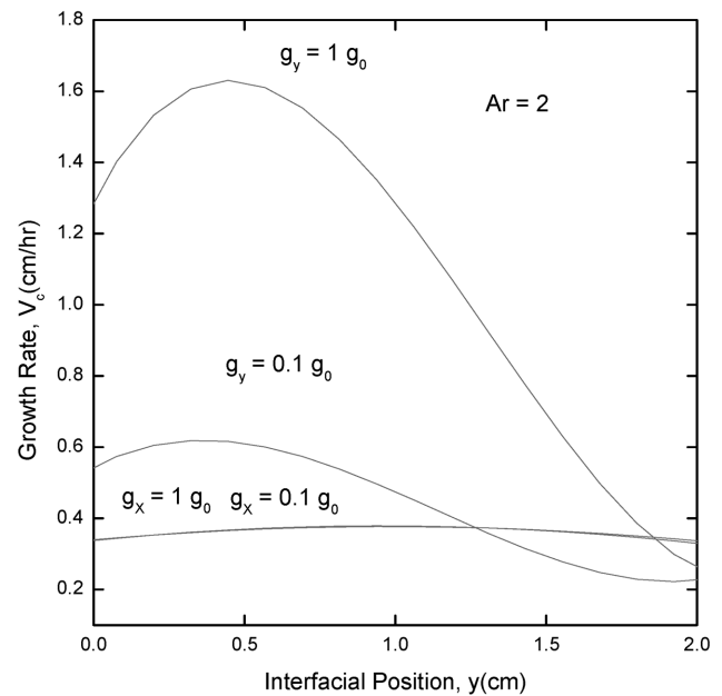
Fig. 5. Interfacial distribution of crystal growth rates for a horizontal ampoule of aspect ratio 2, a linear wall temperature profile between T_s = 612.5 \text{ K} and T_c = 576.0 \text{ K} , and g_y = 1g_0 and 0.1g_0 . Based on Ar=2, Pr=0.86, Le=0.23, Gr_t = 2.14 \times 10^4 , Gr_s = 2.78 \times 10^5 , Pe=2.74, C_v = 1.07 .
