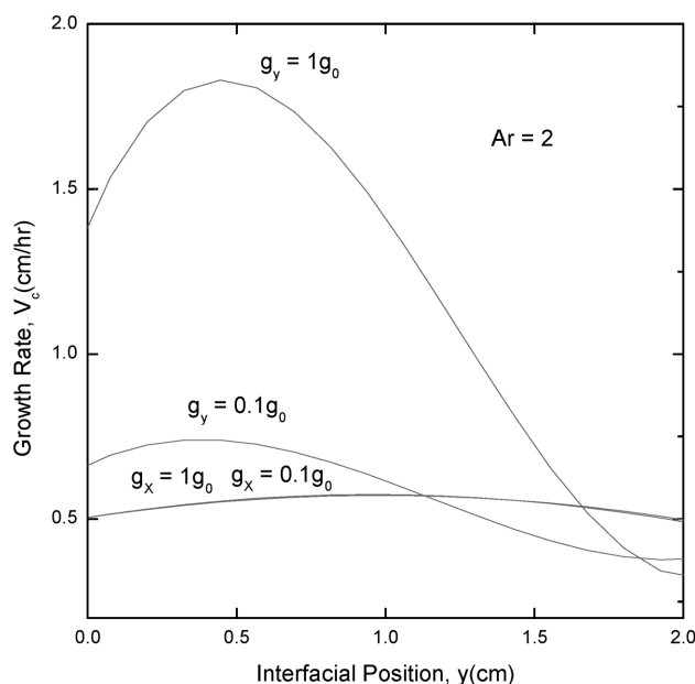
Fig. 14. Interfacial distribution of crystal growth rates for an ampoule of aspect ratio 2, a nonlinear wall temperature profile between T_s = 615.6 K and T_c = 576.0 K, and g_y = 1g_0 and 0.1g_0 . Vertical orientation g_x = 1g_0 .
