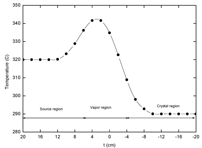
Fig. 9. The nonlinear temperature profile along the ampoule [11].
