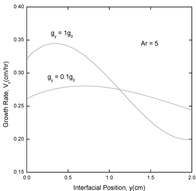
Fig. 13. Interfacial distribution of crystal growth rates for a horizontal ampoule of aspect ratio 5, a nonlinear wall temperature profile between T_s = 612.5 K and T_c = 576.0 K, and g_y = 1g_0 and 0.1g_0 . For the case of g_y = 1g_0 , the corresponding parameters and operating conditions are Ar = 5 , D_{AB} = 0.49 cm 2 s -1 , Pr = 0.82 , Le = 0.33 , Gr_t = 2.65 \times 10^4 , Gr_s = 2.99 \times 10^5 , Pe = 3.74 , C_v = 1.02 .
