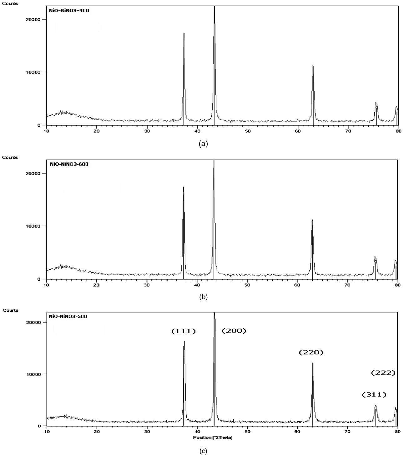
Fig. 1. XRD patterns for the NiO nano crystals synthesized at (a) 900°C, (b) 800°C and (c) 500°C respectively.
