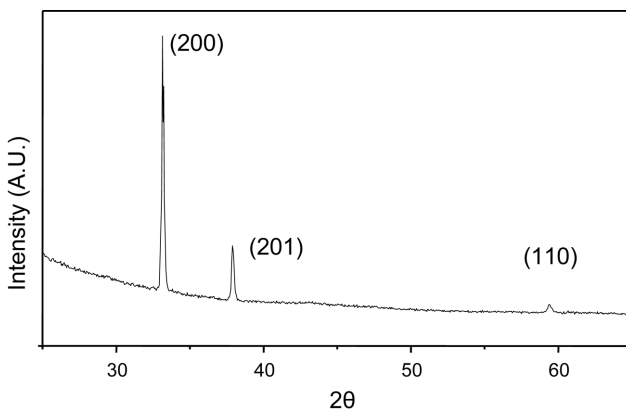
Fig. 1. XRD pattern of the as-grown AlN crystals.
