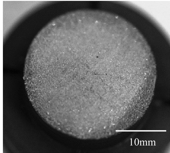
Fig. 2. Photograph of the as-grown AlN crystals.
