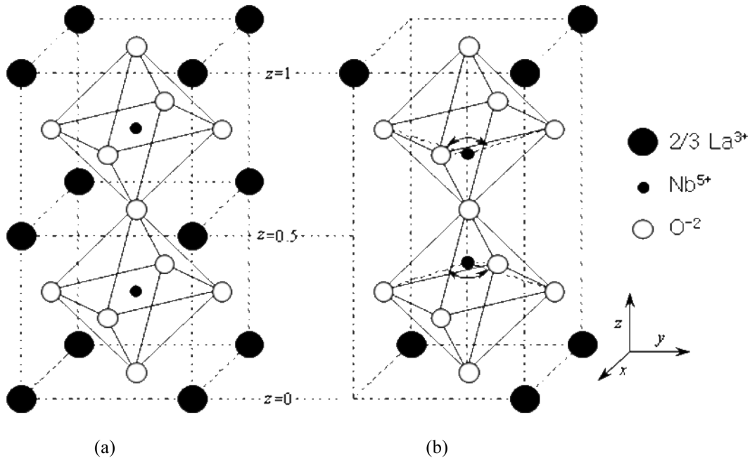
Fig. 1. Comparison of crystal structure in (a) ideal perovskite and (b) A -site defect perovskite of \text{La}_{1/3}\text{NbO}_3 .
