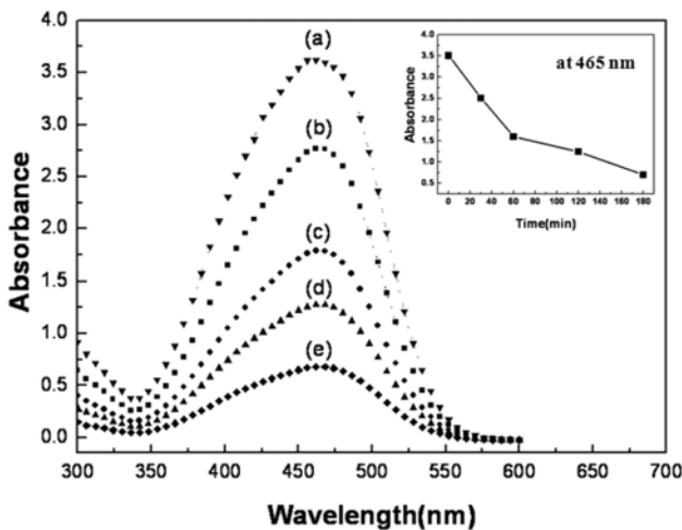
Fig. 6. Photodecomposition of methyl orange by TiO 2 thin film with UV irradiation as a function of immersion time: (a) methyl orange (b) 30 minutes, (c) 60 minutes, (d) 120 minutes and (e) 180 minutes.
