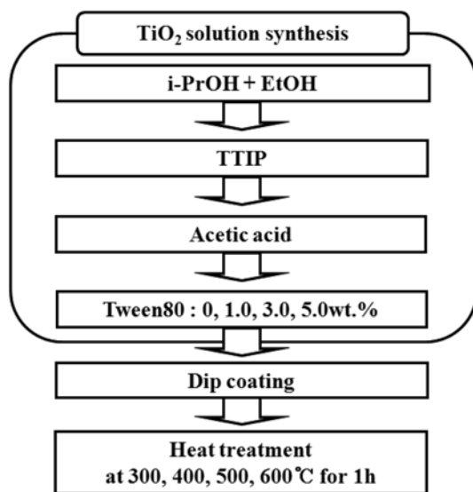
Fig. 1. Flow diagram for fabricating \text{TiO}_2 thin film by a sol-gel method.
