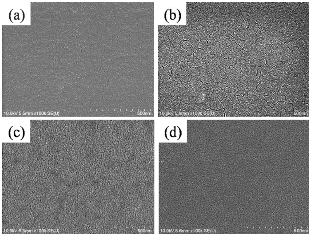
Fig. 2. FE-SEM images of TiO 2 thin films as a function of Tween 80 contents in coating solution: (a) 0.0 wt%, (b) 1.0 wt%, (c) 3.0 wt% and (d) 5.0 wt%.
