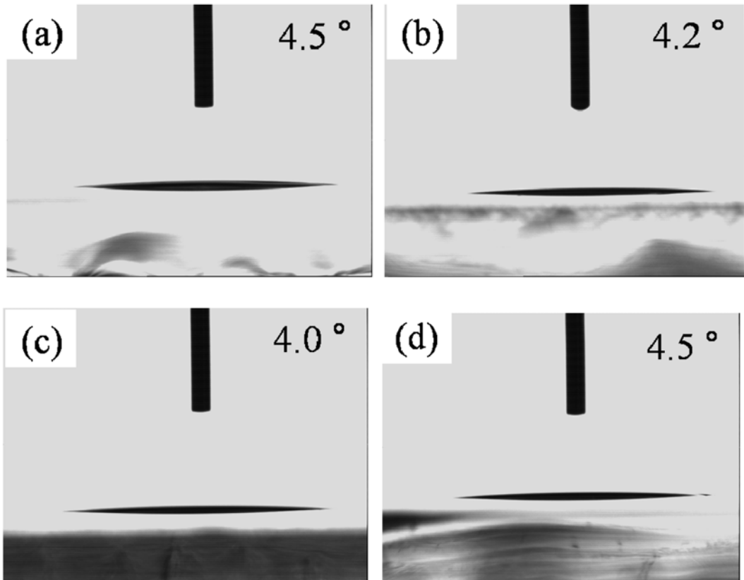
Fig. 5. Contact angles of TiO 2 thin films as a function of Tween 80 contents in coating solution: a) 0.0 wt%, (b) 1.0 wt%, (c) 3.0 wt% and (d) 5.0 wt%.
