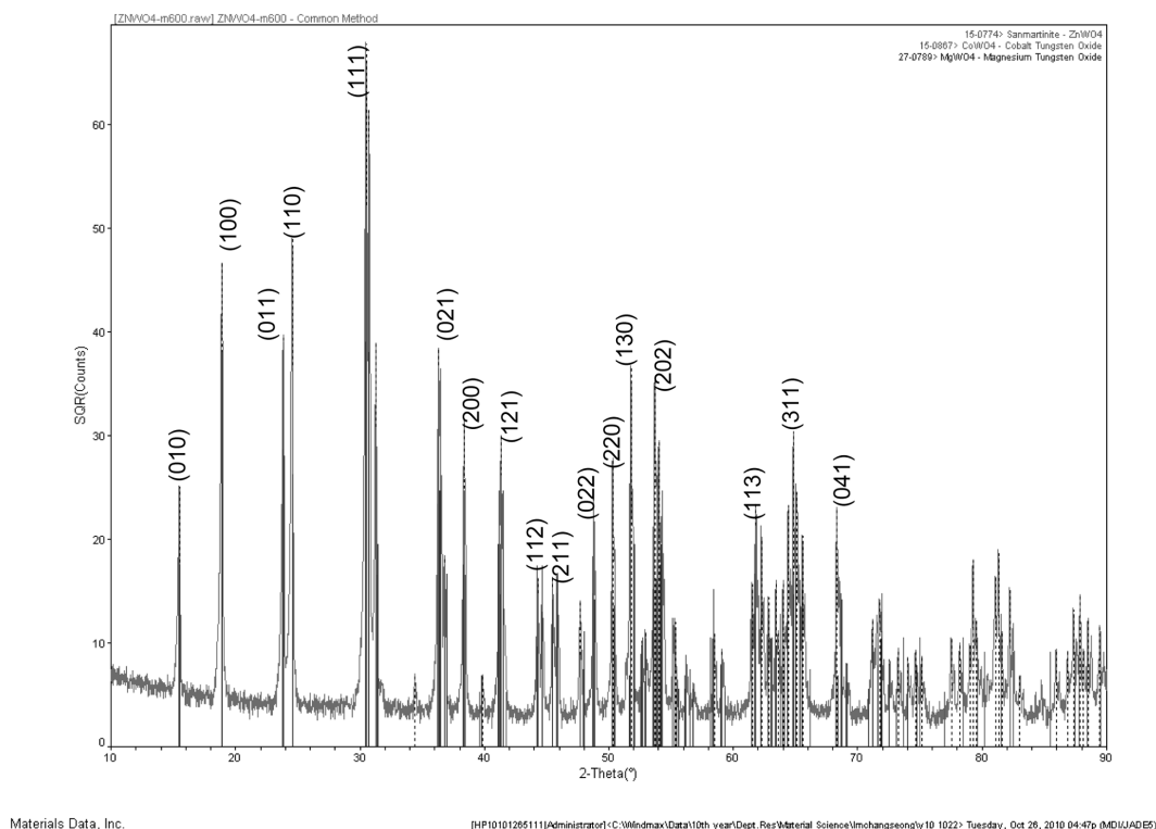
Fig. 1. XRD patterns of the ZnWO 4 particles heat-treated at 600°C for 3 h.
