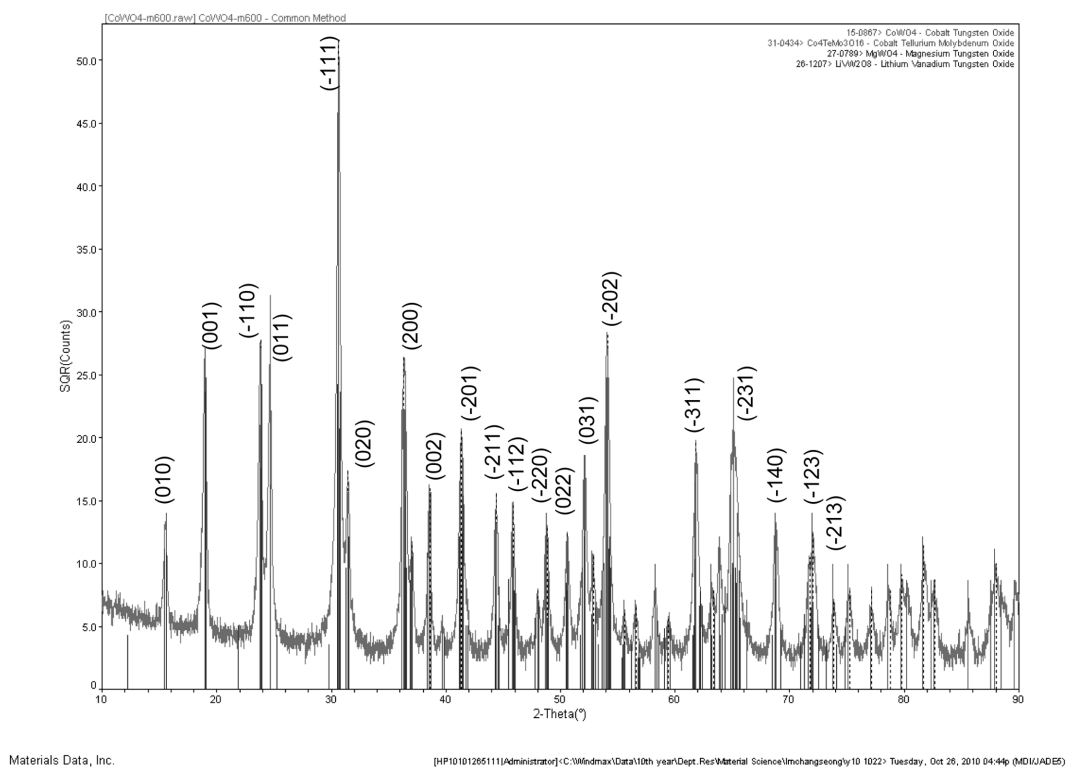
Fig. 2. XRD patterns of the CoWO_4 particles heat-treated at 600^\circ C for 3 h.
