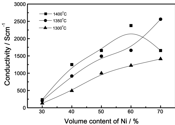
Fig. 3. Electrical conductivity of Ni-YSZ cermets at 1000°C with different amounts of Ni.
