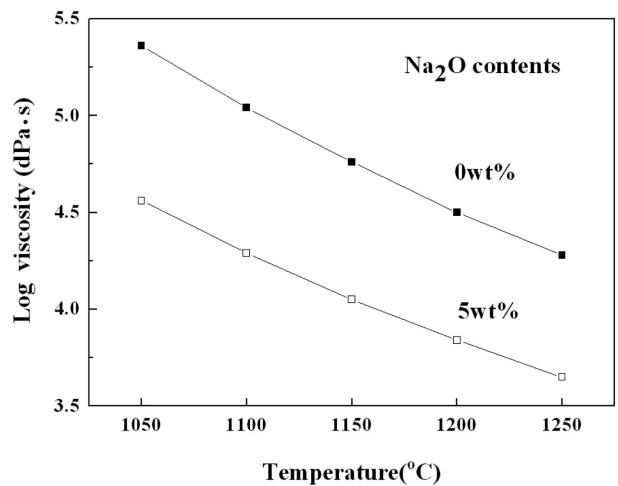
Fig. 2. Log viscosity of the waste glass as a faction of temperature and Na 2 O content added.
