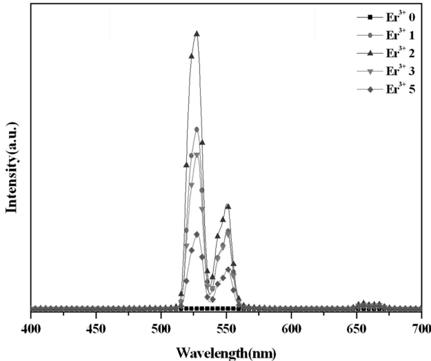
Fig. 3. Photoluminescence spectra of Er 3+ , Yb 3+ co-doped SrMoO 4 with the variation of Er 3+ concentrations.
