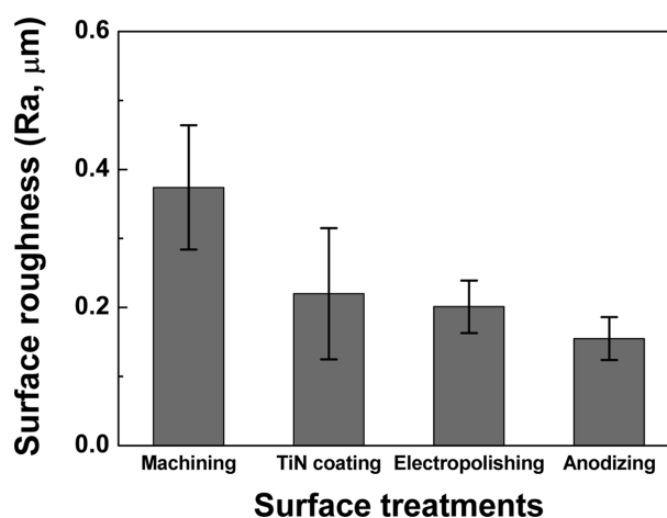
Fig. 3. A comparison of surface roughness (Ra) in various surface-treated Ti membranes.
