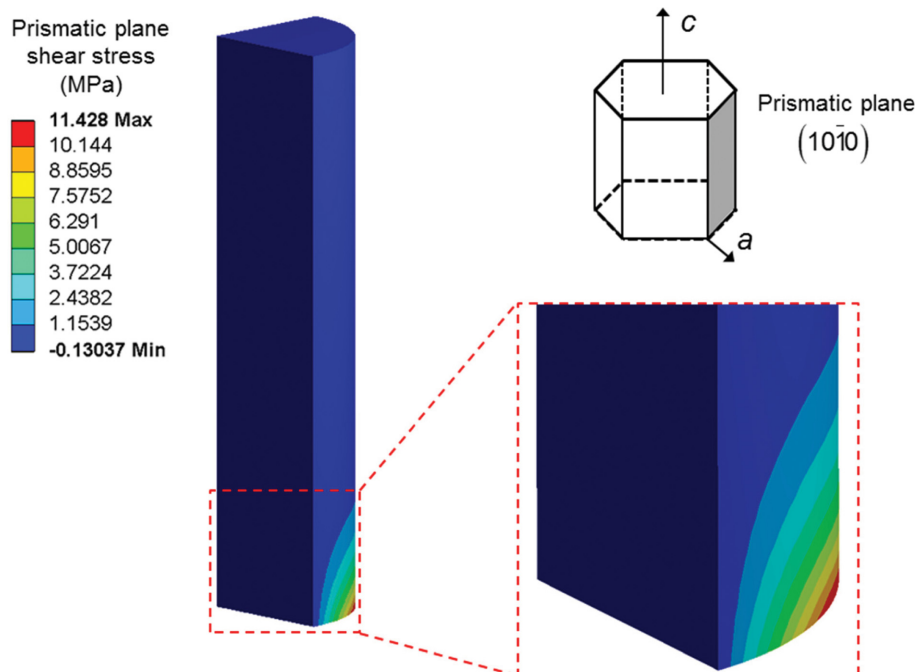
Fig. 4. Shear stress field on xz -plane of as-grown Sapphire with a vertical temperature gradient of 1^{\circ}\text{C}/\text{mm} and a radial (horizontal) temperature gradient of 1^{\circ}\text{C}/\text{mm} . The embedded schematic (upper right side) shows that the xz -plane in the model corresponds to the prismatic plane in c -axis Sapphire growth process.
