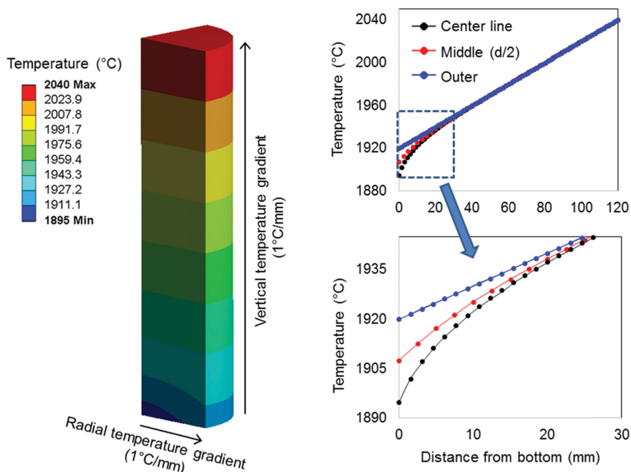
Fig. 2. Calculated temperature field of as-grown Sapphire with a vertical temperature gradient of 1^{\circ}\text{C}/\text{mm} and a radial (horizontal) temperature gradient of 1^{\circ}\text{C}/\text{mm} . The insert is the temperature profiles on the center and the outer line along y-axis, as well as on the middle line in between (on x = d/2 = 12.5 \text{ mm} ).
