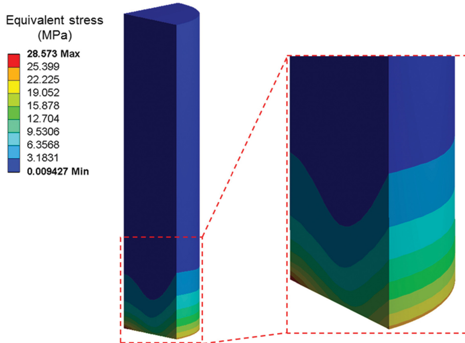
Fig. 3. Equivalent stress field of as-grown Sapphire with a vertical temperature gradient of 1^{\circ}\text{C}/\text{mm} and a radial (horizontal) temperature gradient of 1^{\circ}\text{C}/\text{mm} .
