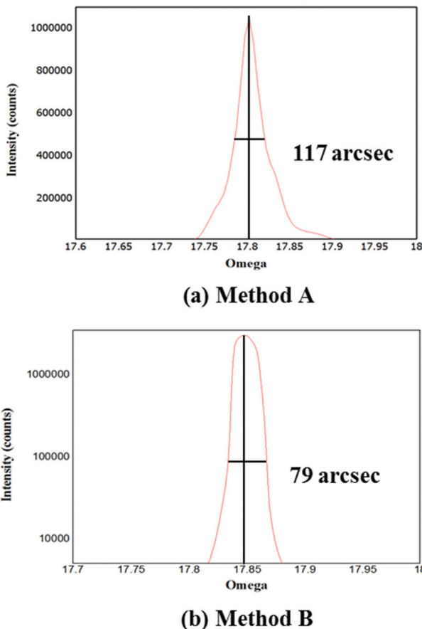
Fig. 7. The full width at half maximum (FWHM) value of vanadium-doped SiC crystal was measured in (a) 117 arcsec and (b) 79 arcsec, respectively.
