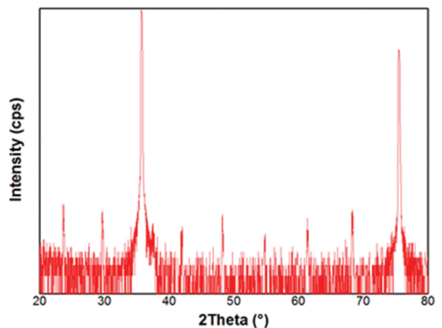
Fig. 3. XRD pattern of vanadium doped SiC crystals.
