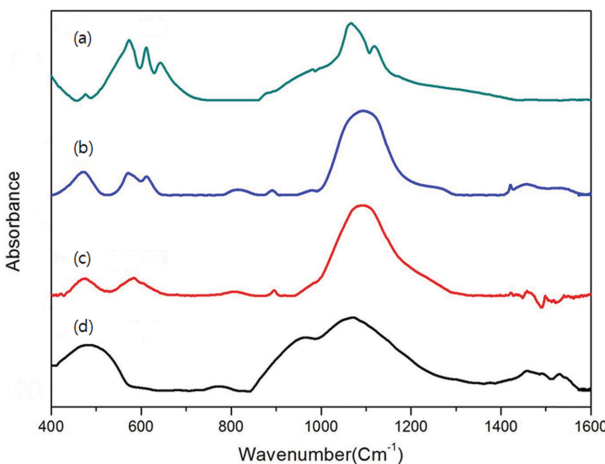
Fig. 3. FTIR spectra of (a) hydroxyapatite, (b) 45S5 after immersion in SBF for 7 days, (c) the coat before immersion in SBF for 7 days, and (d) the coat before immersion in SBF.
