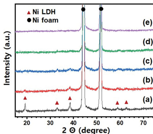
Fig. 1. XRD patterns of the (a) Ni-LDH/NF, (b) 0.01Mo-Ni-LDH/NF, (c) 0.25Mo-Ni-LDH/NF, (d) 0.50Mo-Ni-LDH/NF, and (e) 1.00Mo-Ni-LDH/NF samples.
