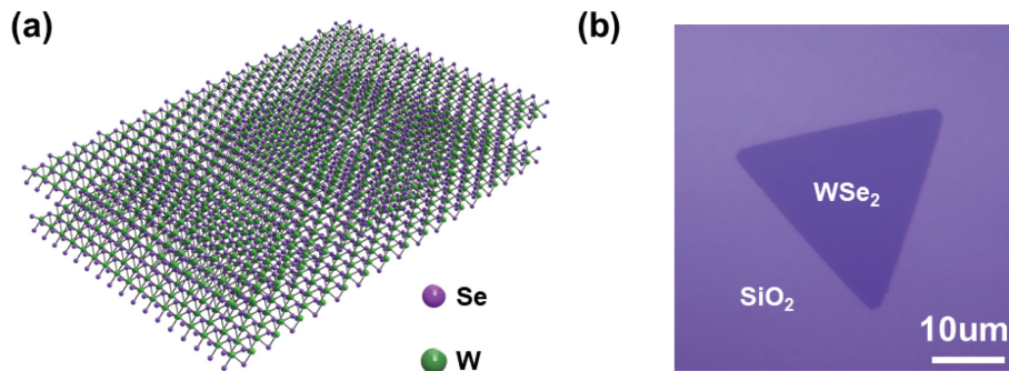
Fig. 1. (a) Schematic diagram of 2H \text{WSe}_2 . (b) Optical image of CVD grown \text{WSe}_2 on \text{SiO}_2 substrate.
