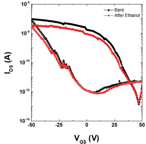
Fig. 4. Log scale of \text{WSe}_2 FET I-V transfer forward (50 V to -50 V) for bare and ethanol exposed samples.
