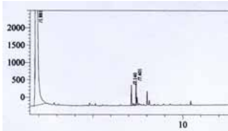
Fig. 10. GC figure of the Yinqiao San with the condenser at the 2 hour after boiling it.
