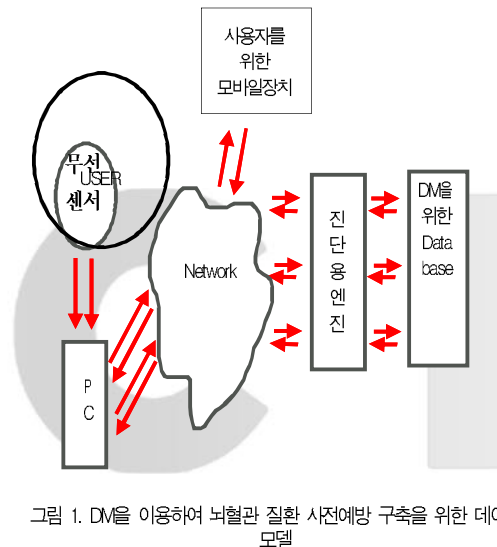
Fig. 1 A data model for system implementation of disease prevention for Ubiquitous Health care prevention using data mining
