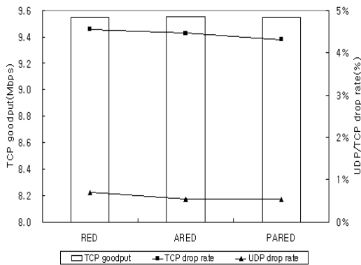
그림 4. TCP goodput과 TCP/UDP 패킷 폐기율 Fig. 4 TCP goodput(left) and TCP/UDP packet drop rate(right)(25 long-lived TCP connections with 10% UDP traffic)
