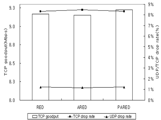
그림 5. TCP goodput과 TCP/UDP 패킷 폐기율 Fig. 5 TCP goodput and TCP/UDP packet drop rate(50 long-lived TCP connections with 10% UDP traffic)
