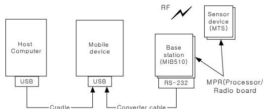
Fig. 10. Configuration of Development System and Equipments
