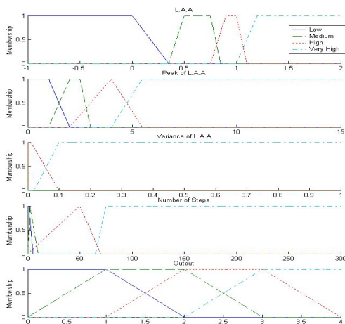
Fig 8. Membership for inputs and output
