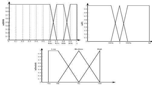
Figure 4. Fuzzy values of fuzzy variables DBAH, DF, and Threshold
