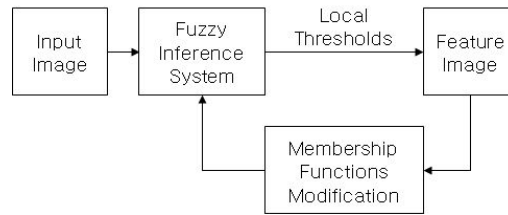
Figure 3. the overall process for color sketch feature map.
