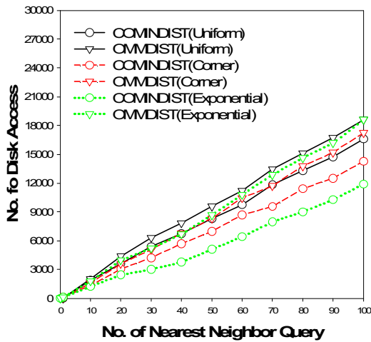
(b) 질의크기=1.0%
