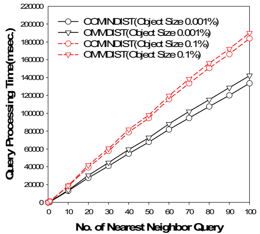
(a) 균일분포
