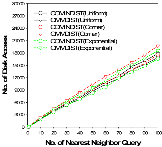
(a) 질의크기=0.01%
