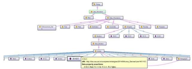
Fig. 20. Graph of Legal Ontology Construction
