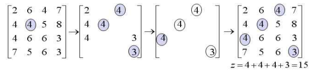
Fig. 3. The Solution of SM_1 Problem Using TA
