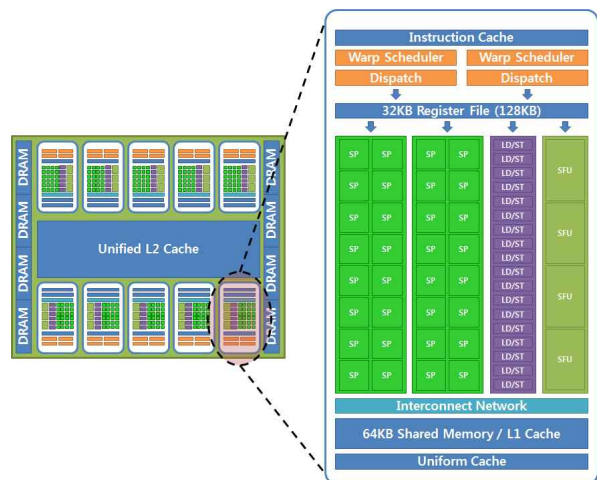
Fig. 1. NVIDIA's GPU architecture(Fermi)
