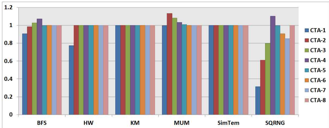
Fig. 3. GPU performance according to number of CTAs assigned to the SM
