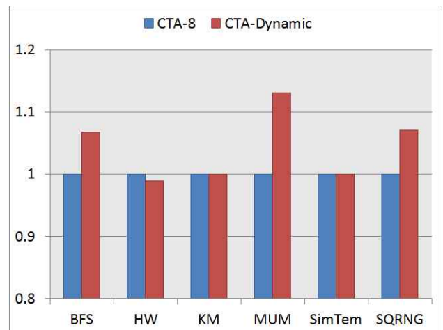
Fig. 4. GPU performance according to IPC-based Dynamic CTA Scheduling Scheme
