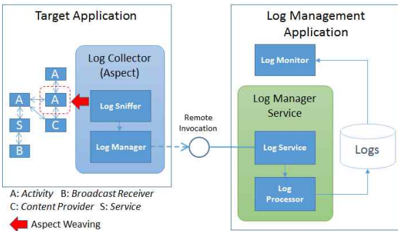
Fig. 1. Log Service Management Model
