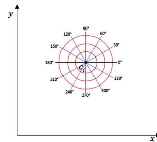
Fig. 5. Polar coordinate centered at c_i
