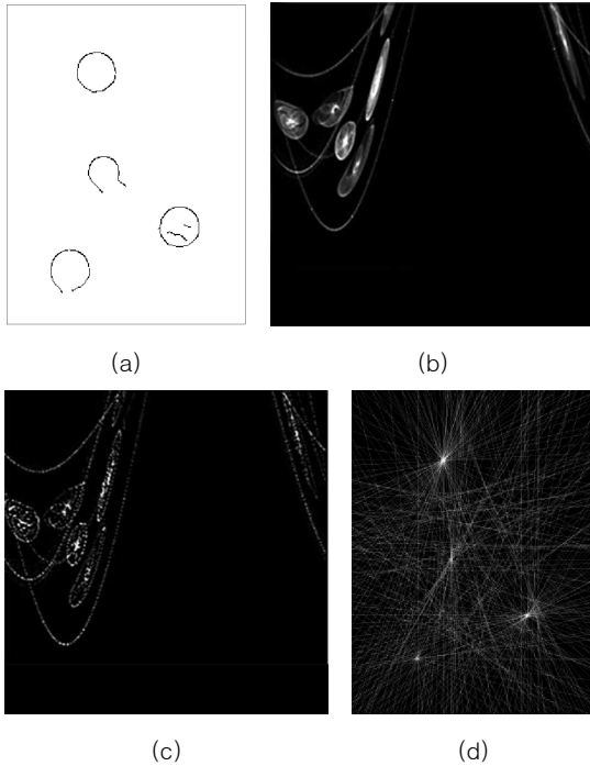
Fig. 4. (a) Edges of an image (b) Parameter histogram built in (\theta, \rho) space. (c) Extracted ridges (d) Detected circle centers.
