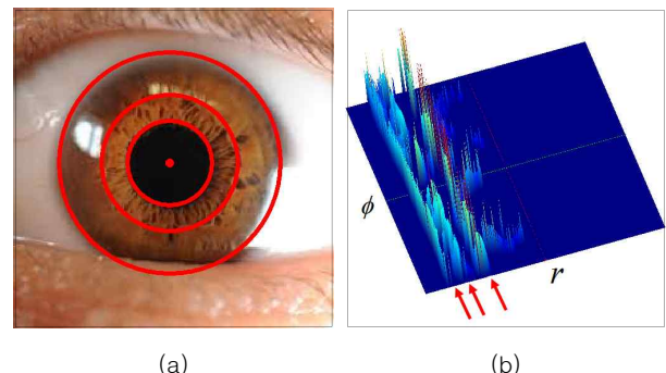
Fig. 6. (a) 3 concentric circles detected. (b) p_i[r][\phi] table for image (a).
