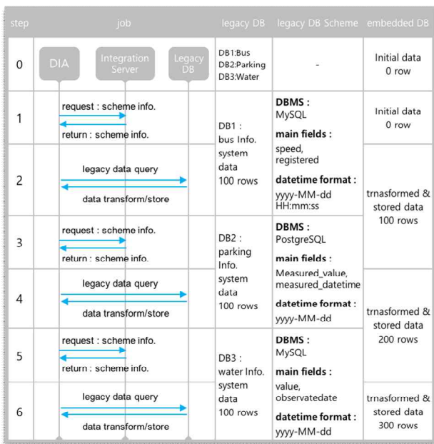
Fig. 7. Flow of Data Translation Test
