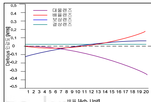
Fig 2. The graph of optical sensitivity analysis
