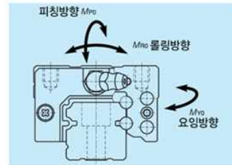
Fig. 9. The direction of moment on LM Block
