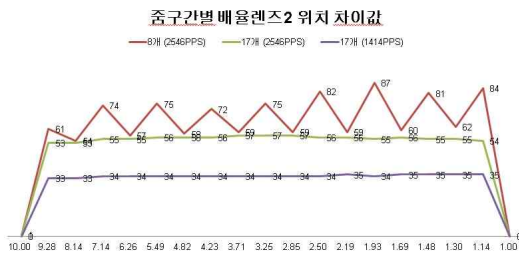
Fig. 14. The position difference of magnification lens 2 by zoom points
