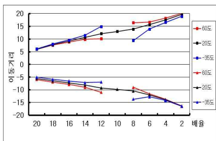
Fig 4. The optical path graph on temperature in camera 1
