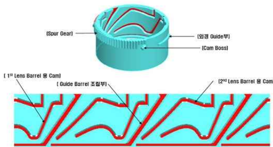
Fig. 8. The barrel on including the optical path
