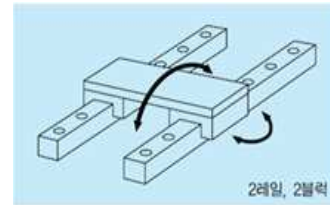
Fig. 10. The structure of 2 Rail and 2 Block
