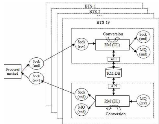
Fig. 3. Simulation Scenario
