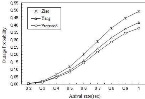
Fig. 4. Outage Probability
