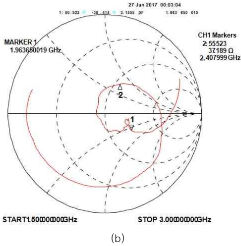
Fig. 4. Measured curves. (a) VSWR (b) Impedance Locus
