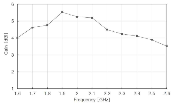
Fig. 6. Measured Gain.
