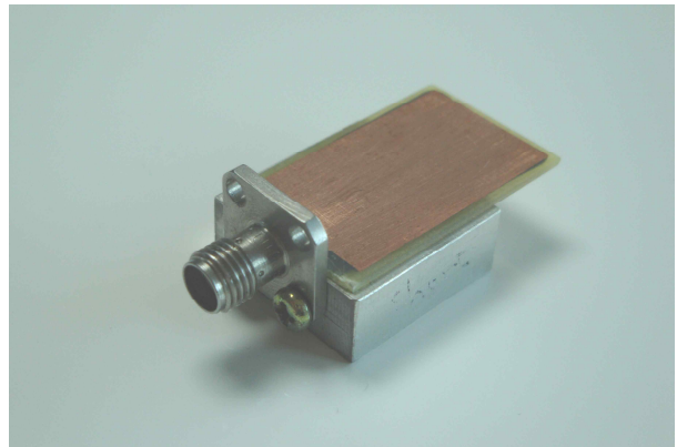
Fig. 3. Fabricated Microstrip Antenna.
