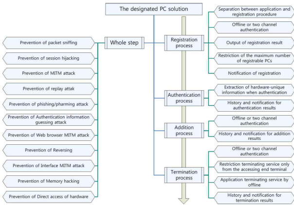
Fig. 7. Whole model applying security requirements
