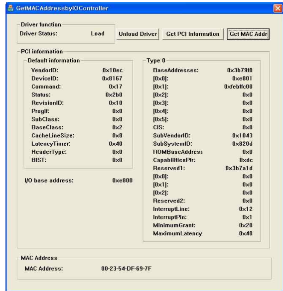
Fig 5. Example of extracting MAC address using I/O controller
