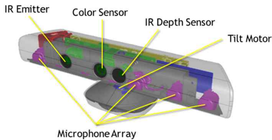
Fig. 1. Kinect Sensor
