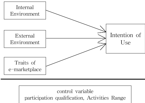
Fig. 1. Research Model
