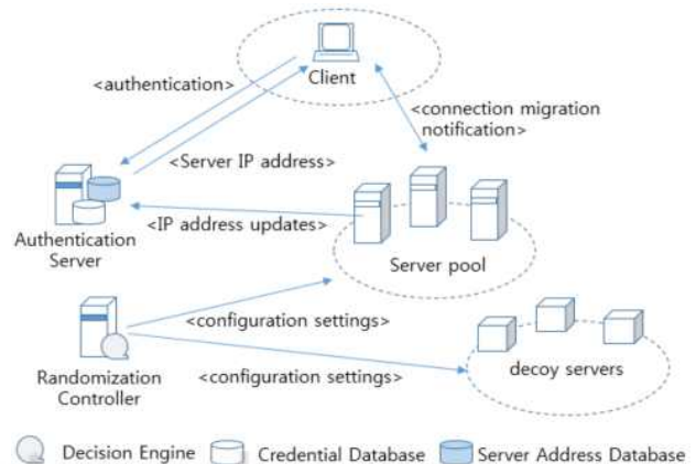
Fig. 4. DESIR architecture
