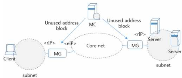
Fig. 3. RHM architecture
