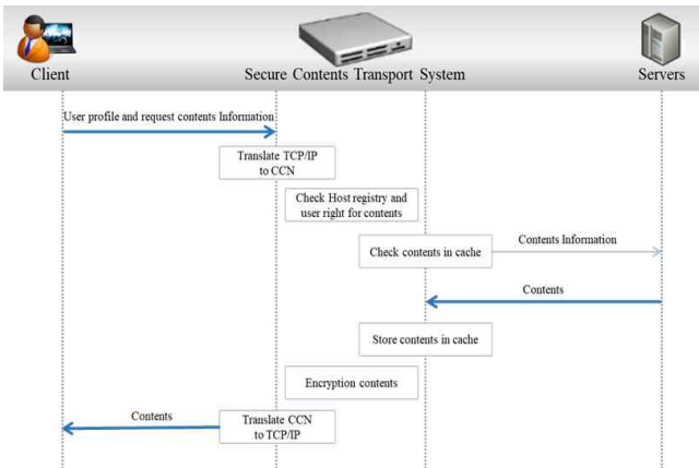
Fig. 5. Operating Flow
