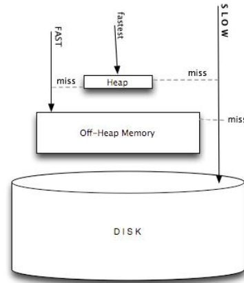
Fig. 7. Comparison Heap and Off-heap[15]
