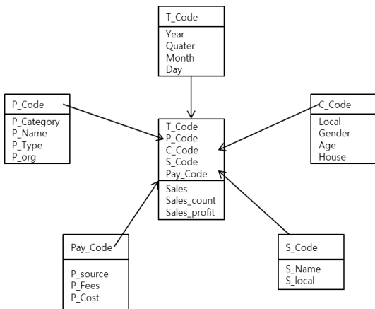
Fig. 3. Conceptual Star Schema
