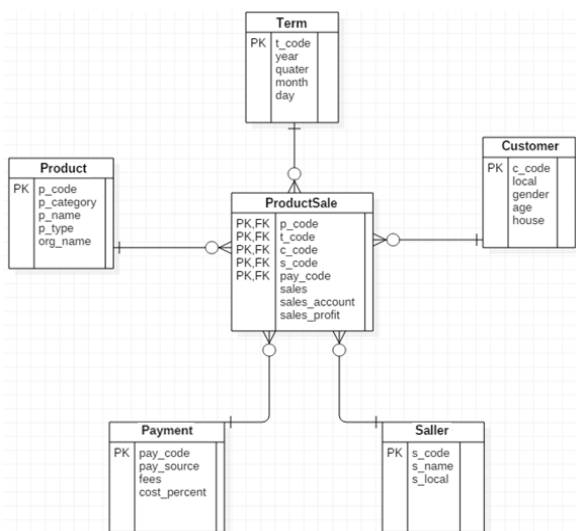
Fig. 5. Logical Star Schema
