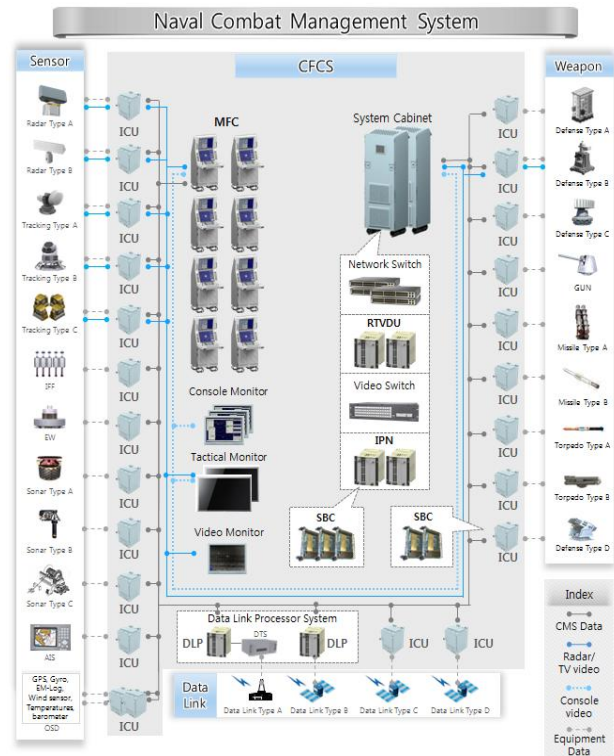
Fig. 1. Naval CMS architecture
