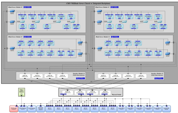
Fig. 8. Server Virtualization Architecture
