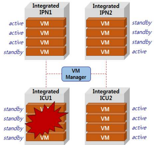
Fig. 5. Redundancy method of Integrated equipment
