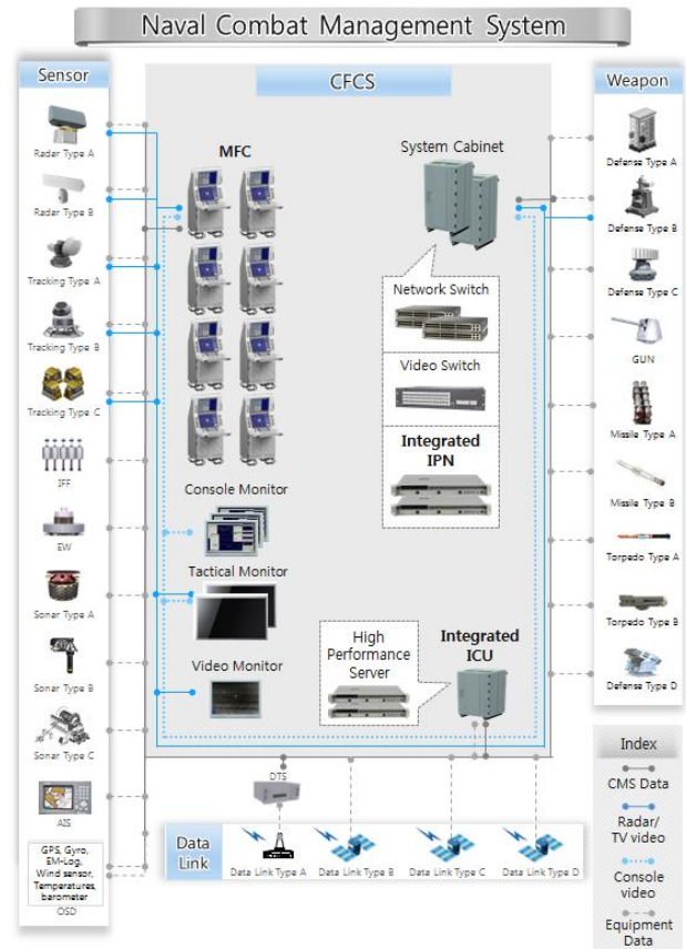
Fig. 3. Virtualization based naval CMS architecture
