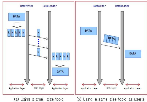
Fig. 4. Comparison for message sending and receiving methods
