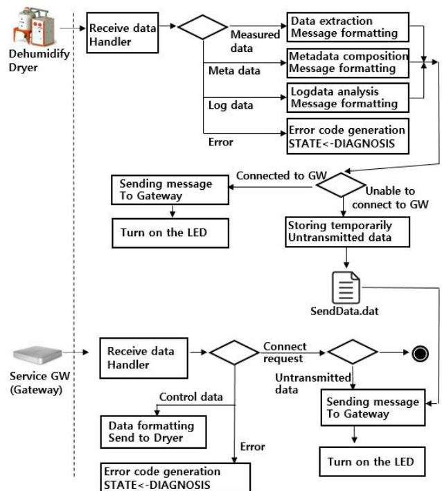
Fig. 4. Activity diagram for the interface module
