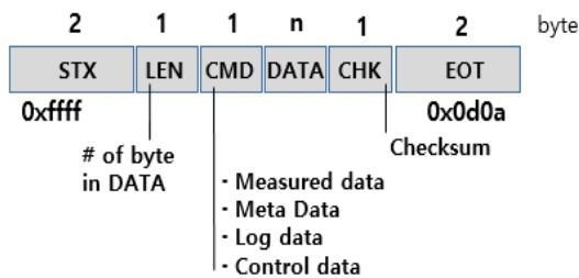
Fig. 5. Data format between dryer and interface module
