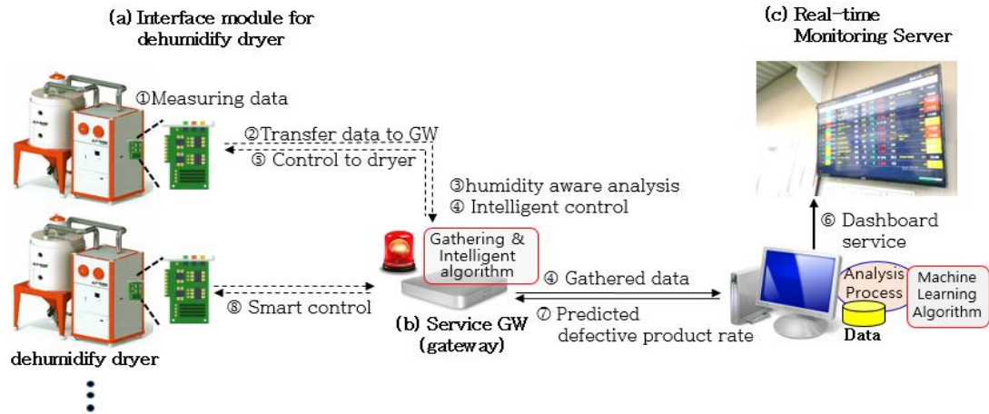
Fig. 2. Smart Factory System Model for Plastic Molding System
