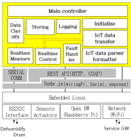
Fig. 3. Software Configuration of Interface Module for Dehumidify Dryer
