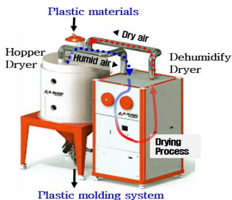
Fig. 1. Dehumidify Dryer in Plastic Molding System
