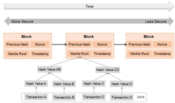
Fig. 1. Blockchain structure
