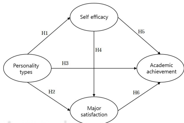
Fig. 3. Research Model
