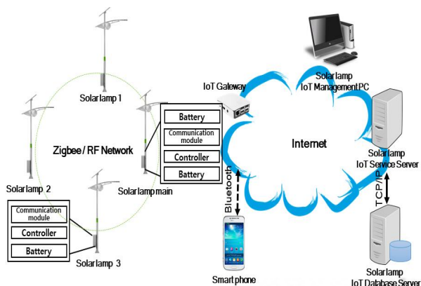
Fig. 1. IoT based monitoring and control system
