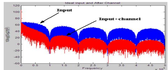
Fig. 13. Power spectrum vs Frequency
