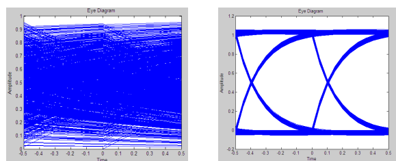
Fig. 20. input 1Gbps (a) Eye diagram of Before equalization (b) eye diagram of after equalization
