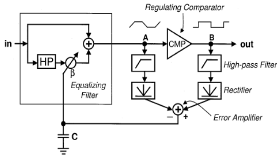
Fig. 10. Block Diagram of conventional Continuous-time adaptive Cable equalizer[15]
