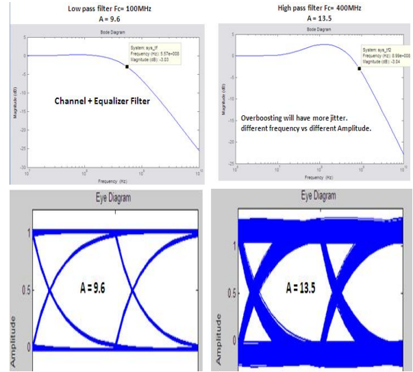
Fig. 12. input 1Gbps (a) magnitude response vs Frequency (b) eye diagram of after equalization
