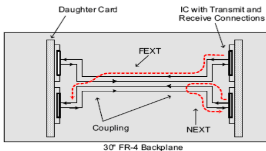
Fig. 2. Channel-Backplane
