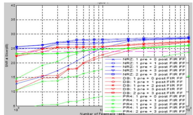
Fig. 3. Performance comparison of NRZ, DB, and PR4 signaling over Tyco channel #1 with data rate of 10.3Gb/s with the worst case NEXT[2]
