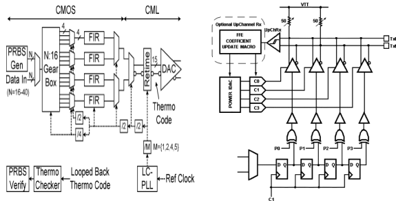
Fig. 4. Typical TX pre-emphasis schemes
