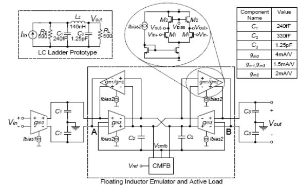
Fig. 7. 3 rd order delay Cell
