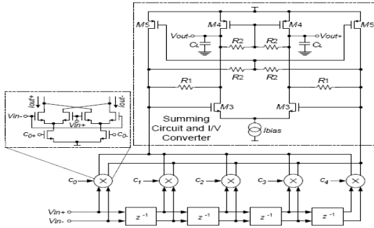
Fig. 8. Summing Circuit and I/V Converter
