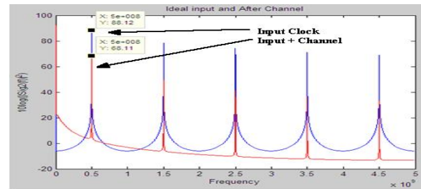
Fig. 17. Power spectrum vs Frequency input and input+channel
