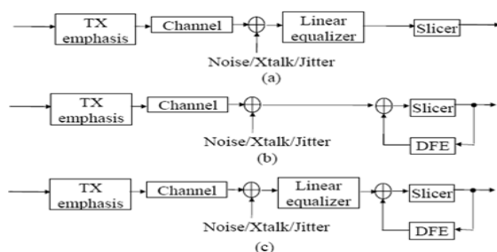
Fig. 5. Different Equalization Schemes: (a) LE; (b) DFE; (c) LE+DFE.[2]
