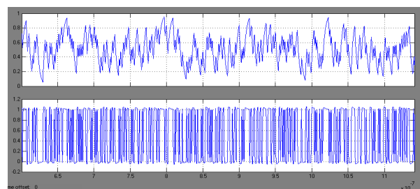
Fig. 19. Transient simulation (a) up part TX+ Channel (b) down TX+Channel+Equalizer filter
