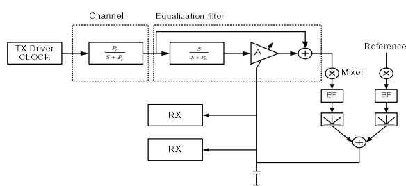
Fig. 16. Block Diagram of Continuous-time adaptive Cable equalizer with Clock
