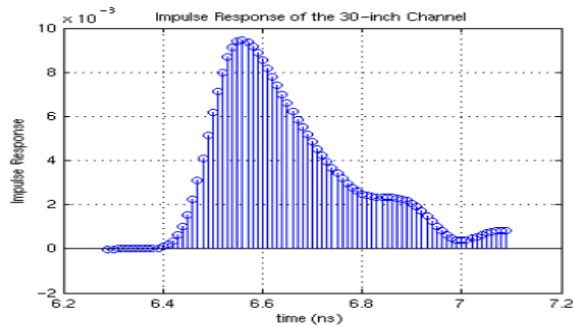
Fig. 1. Normalized impulse response of a 30 inch FR-4 backplane channel[1]
