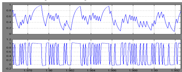
Fig. 15. Transient simulation (a) up part TX+Channel (b) down TX+Channel+Equalizer filter
