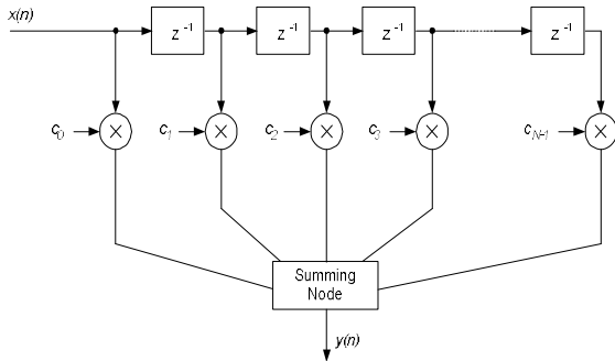
Fig. 6. 5-tap transversal equalizer structures
