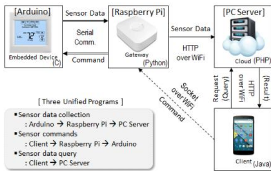
Fig. 2. Example of Home Monitoring System
