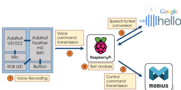
Fig. 3. Voice Command to Text Conversion Procedure
