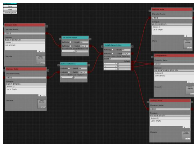
Fig. 4. Dialogue Node Graph for Story
