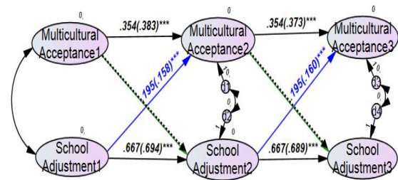
Fig. 3. Paths of Autoregressive cross-lagged model
