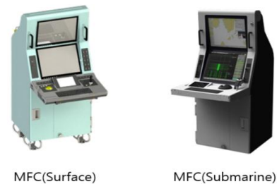
Fig. 1. Naval Combat System Multi Function Console Mockup Image
